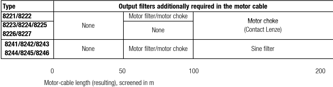
FIG 4-7 Output filters additionally required in the motor cable
