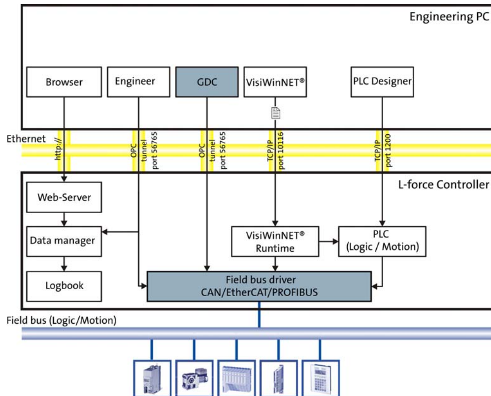
[4-1] Exemplary system overview with an Engineering PC and an L-force Controller
