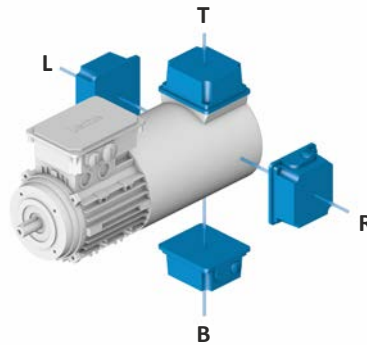
Blower terminal box with/without M23 connector
