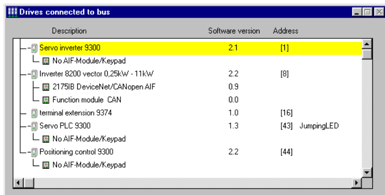
Window Drives connected to bus
