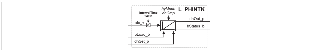
Integration (L_PHINTK)
