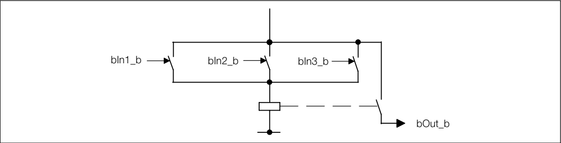
Fig. 2-44 Function of L_OR as a parallel connection of normally-open contacts
