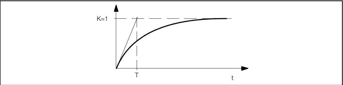
Fig. 2-25 Delay T of the first-order delay element
