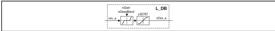
Dead band (L_DB)
