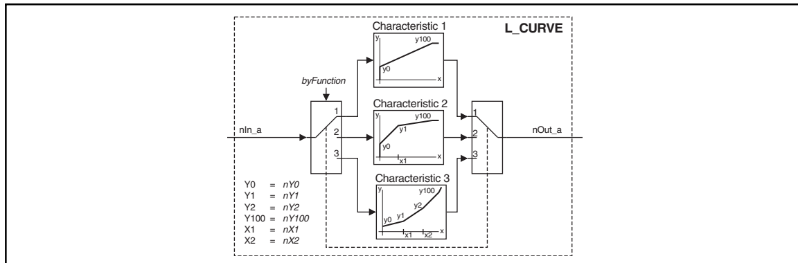
Curve function (L_CURVE)
