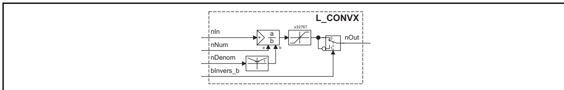
Conversion (L_CONVX)
