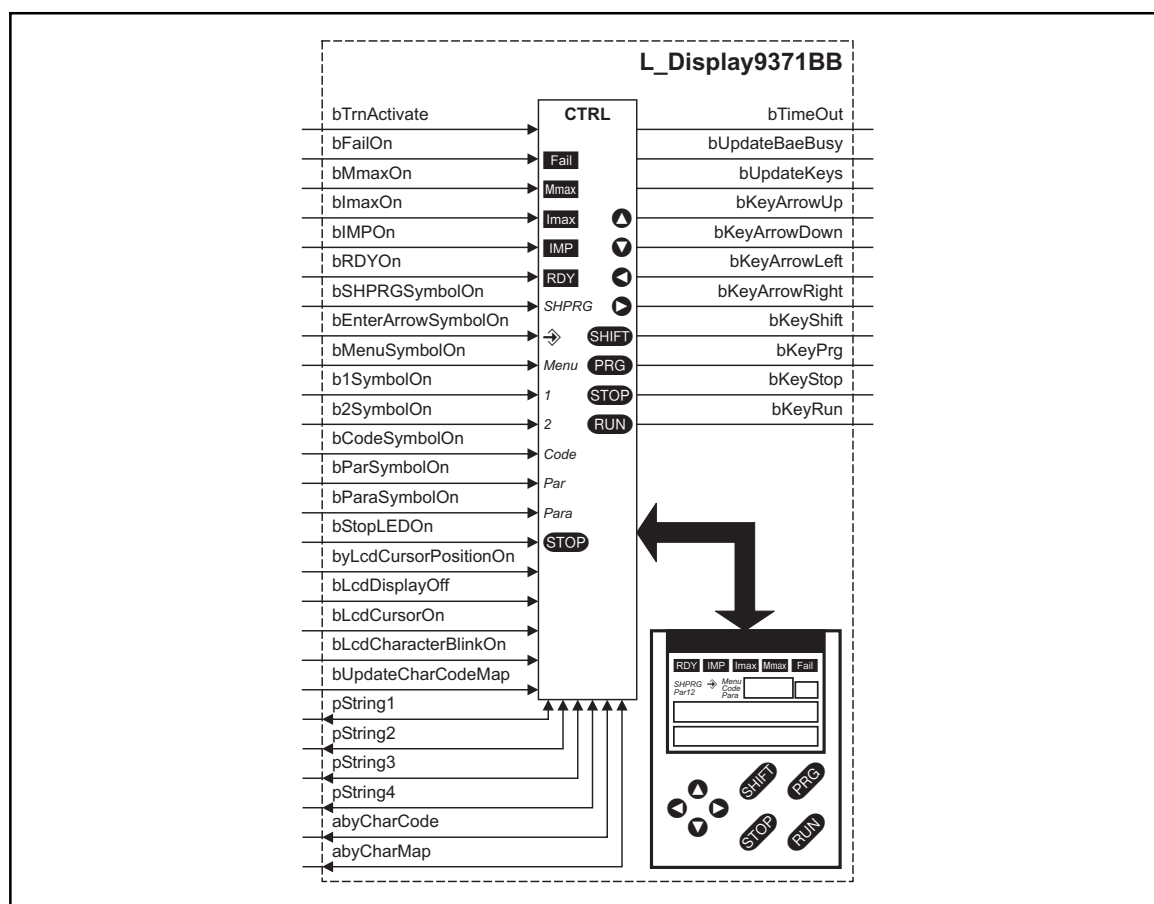
FB L_Display9371BB
