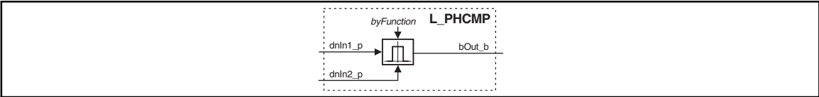
Fig. 2-51 Comparison (L_PHCMP)
