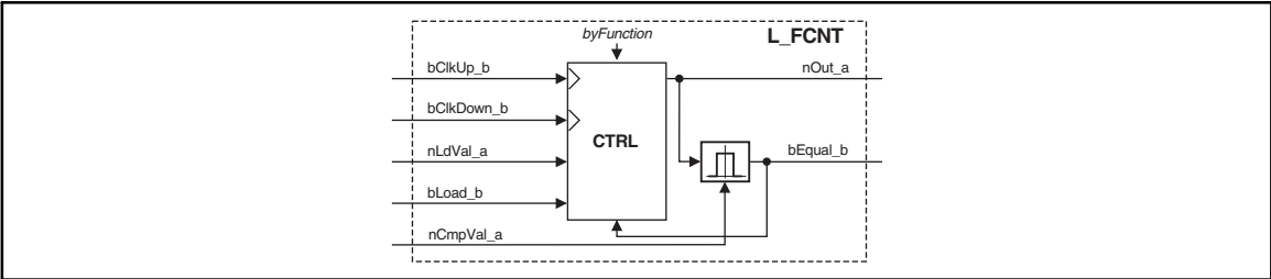
Fig. 2-38 Up/down counter (L_FCNT)
