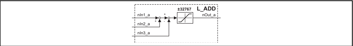
Addition (L_ADD)
