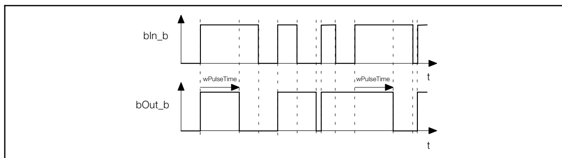
Evaluation of FALSE-TRUE transitions
