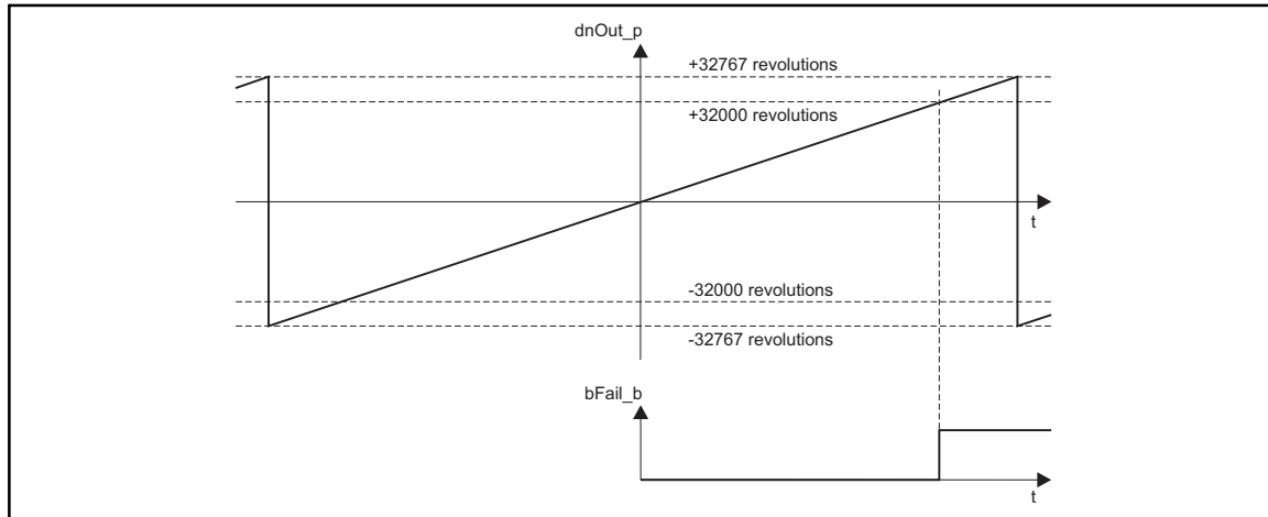
Function of L_PHINT with constant input value
