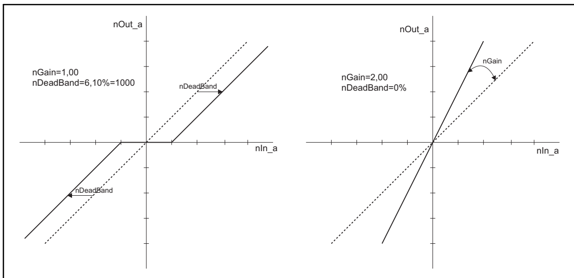
Dead band and gain
