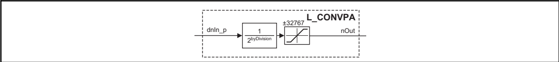
Conversion of phase-angle to analog (L_CONVPA)
