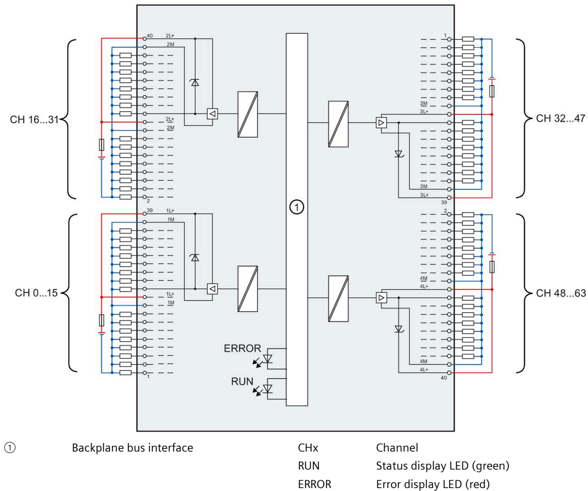
Figure 3-1 Block diagram and terminal assignment
