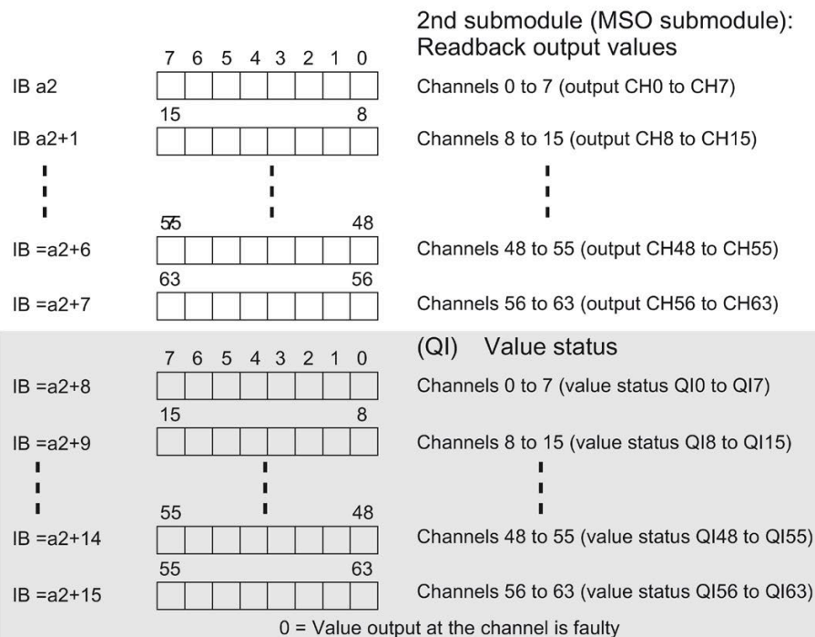
Figure 4-3 Address space for configuration as 1 x 64-channel DQ 64x24VDC/0.3A BA MSO with value status
