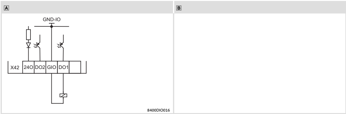
Fig. 6-7 Wiring examples of the digital inputs and outputs A Digital control (relay, valve, ...) with internal 24 V supply B - X42 Plug for the digital outputs (configured) GIO Ground reference potential for the digital inputs and outputs (GND-IO)
