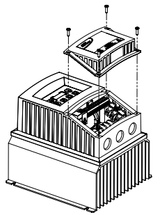
Figure 1: Remove Cover
