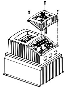
Figure 3: Replace Potentiometer as SMV Terminal Cover
