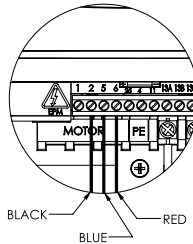
Figure 2: Wiring Potentiometer to SMV Terminal Strip
