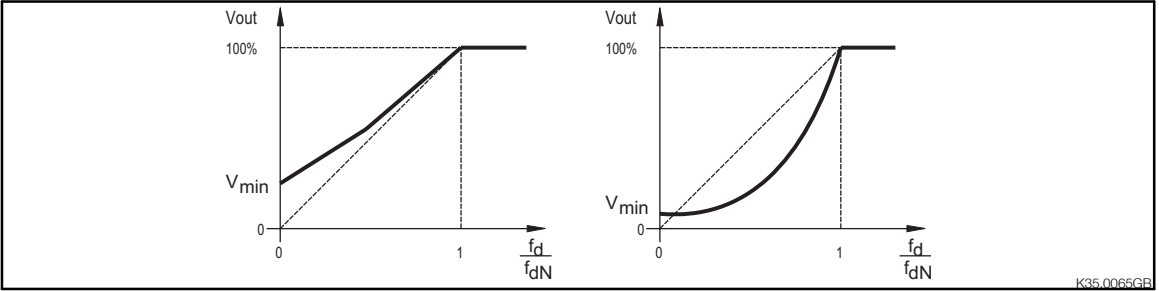
C014 = -2- Linear characteristic
