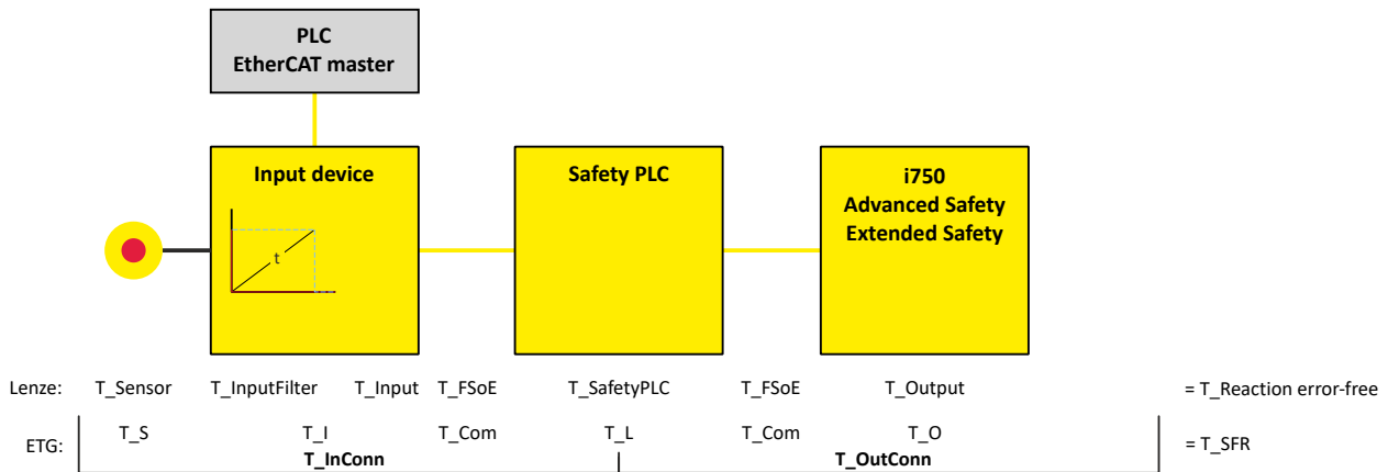
Fig. 20: Maximum response time with error-free communication without Safe Brake Control (SBC)
