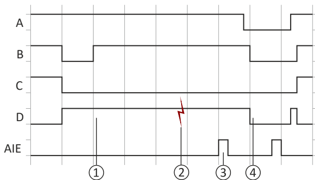
Fig. 14: Contact function test – faulty input signals
