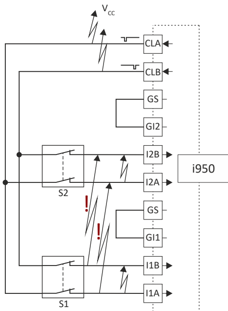
Fig. 11: Ways to detect errors
