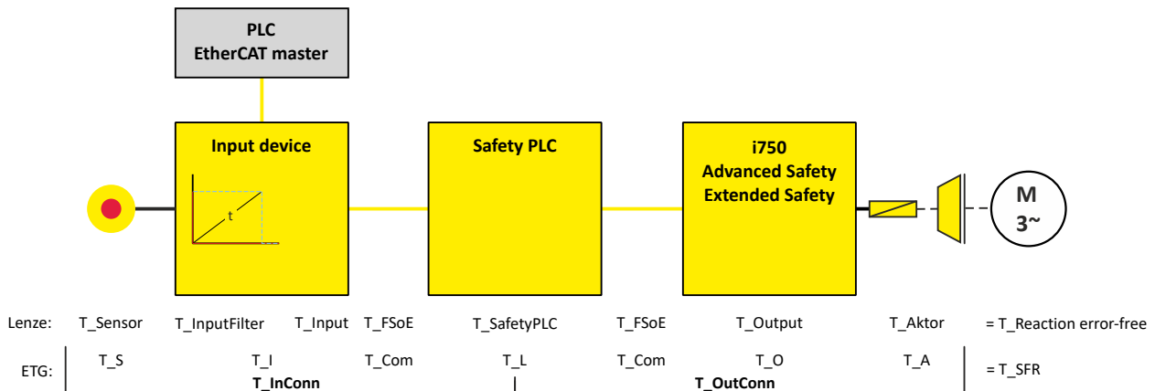
Fig. 21: Maximum response time with error-free communication with Safe Brake Control (SBC)
