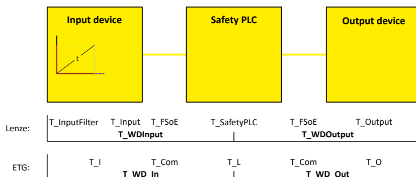
Fig. 22: FSoE watchdog time
