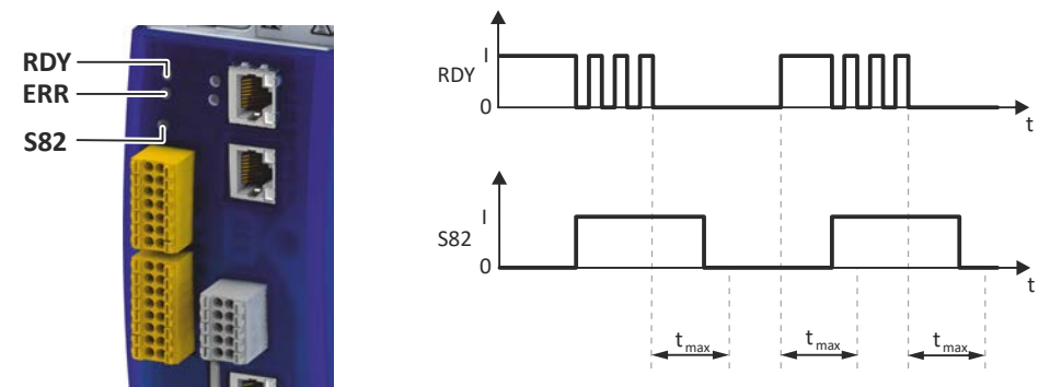
Fig. 10: Sequence of the acknowledgement procedure
