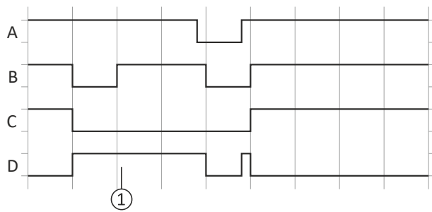
Fig. 13: Contact function test – error-free input signals
