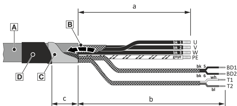
Fig. 8: Cable assembly
