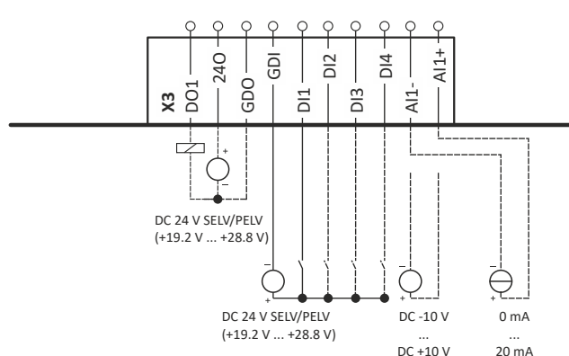
Fig. 7: Wiring diagram of control connections
