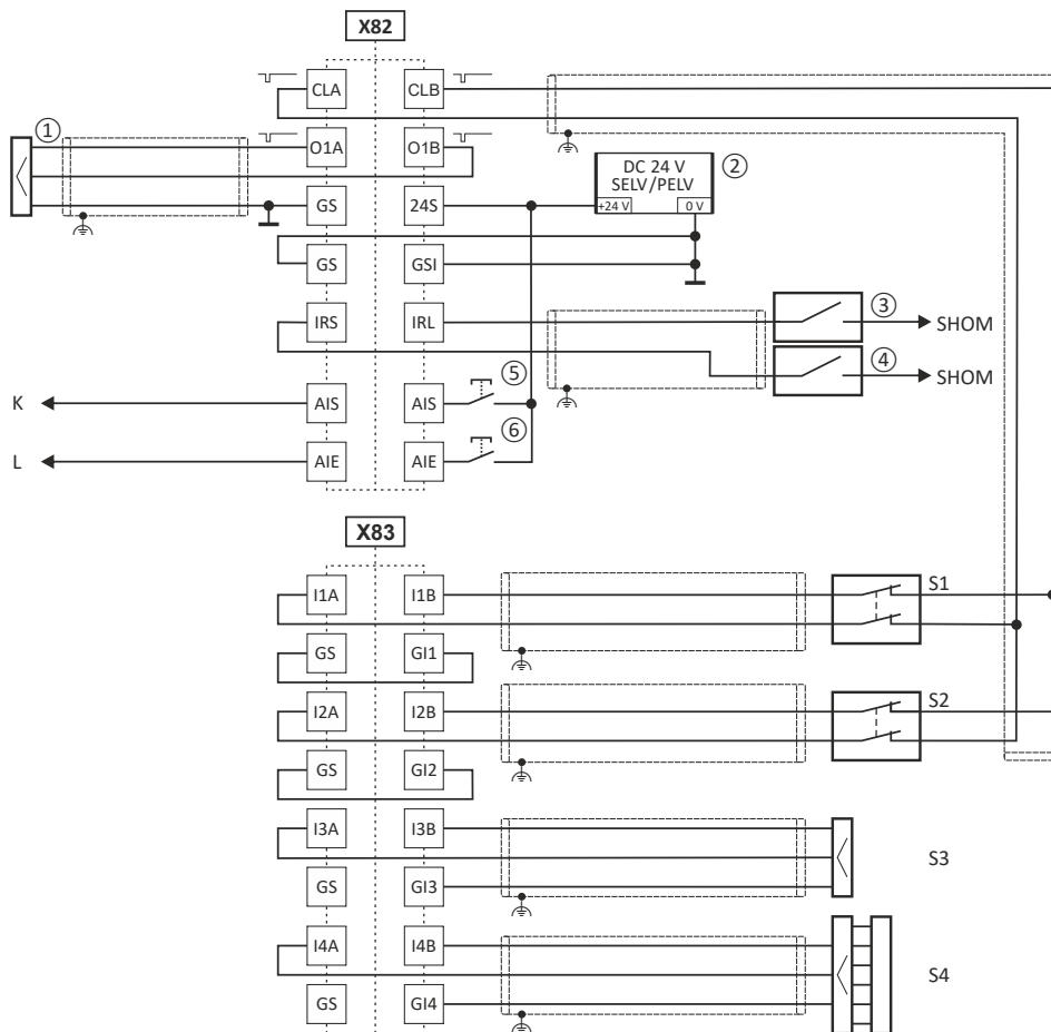
Fig. 9: Sample circuit
