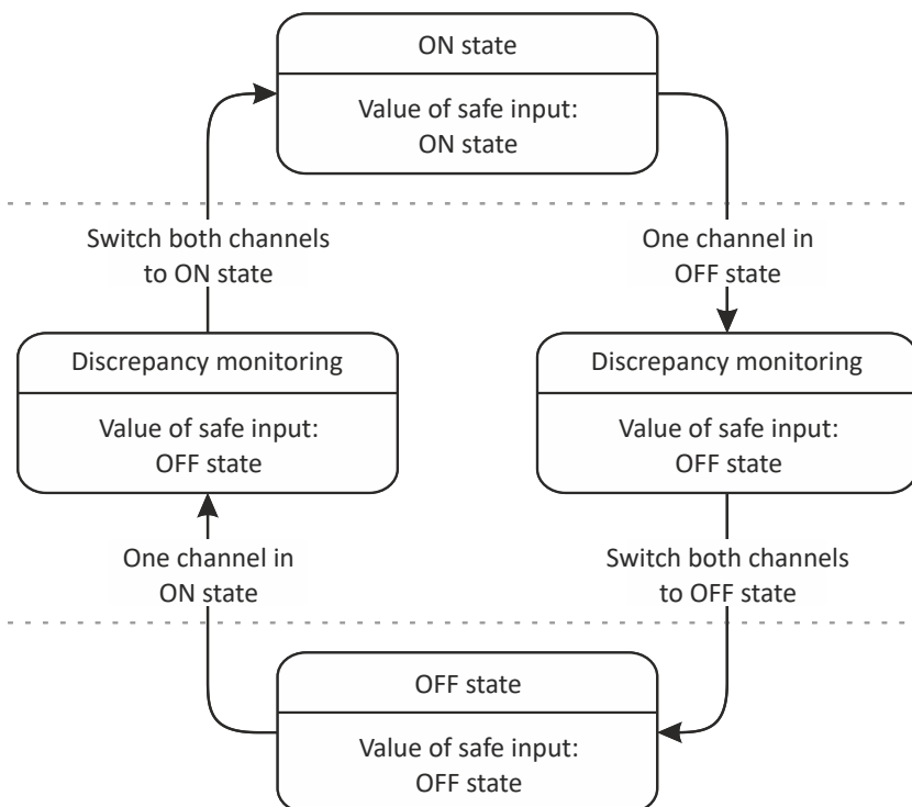
Fig. 12: Contact function test – state behavior
