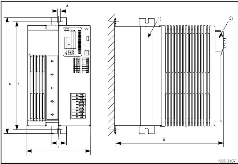
FIG 4-2 Dimensions 8215 - 8218: Standard assembly 1) Fixing rail for side assembly 2) Observe the free space required for the connection cables 3) With attachable fieldbus or I/O module: Observe assembly depth and assembly space required for connection cables
