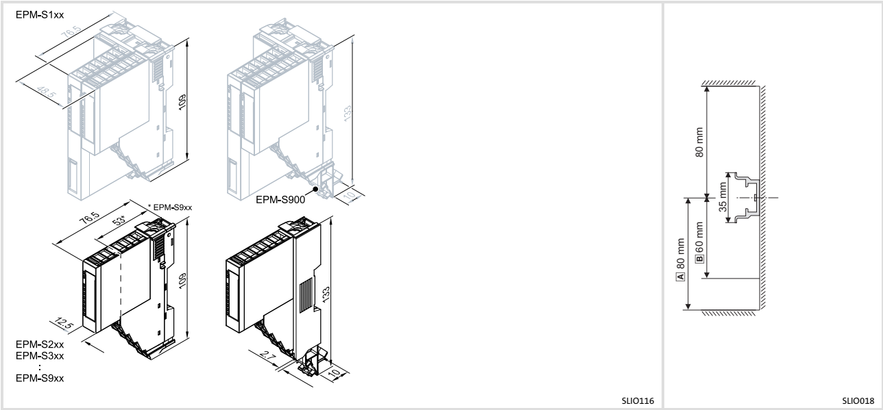
[A] Mounting clearance without shield bus [B] Mounting clearance with shield bus
