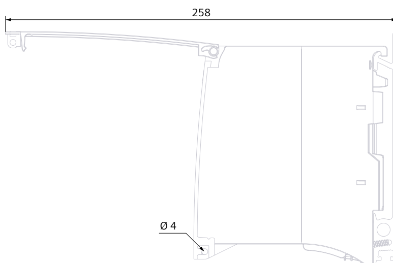
Figure A-2 Dimension drawing of CPU 1515R-2 PN, side view with open front cover
