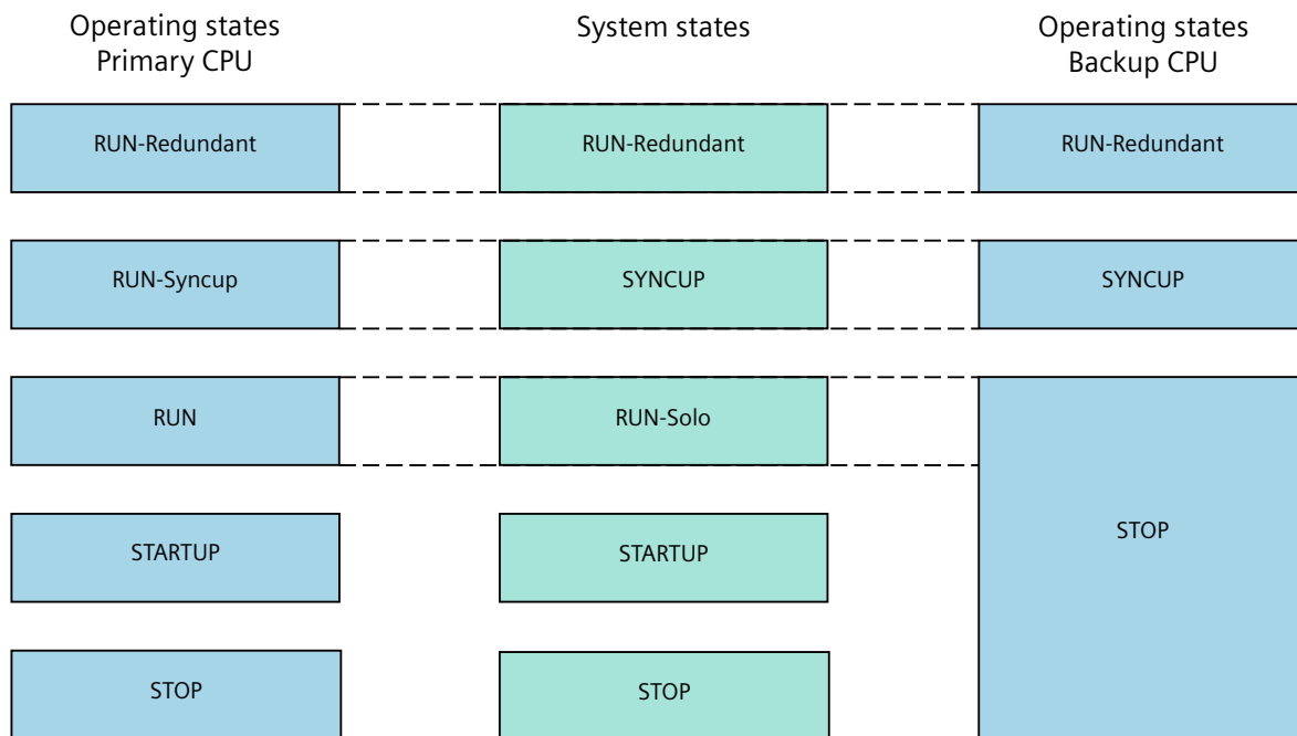
Figure 5-2 Operating and system states
