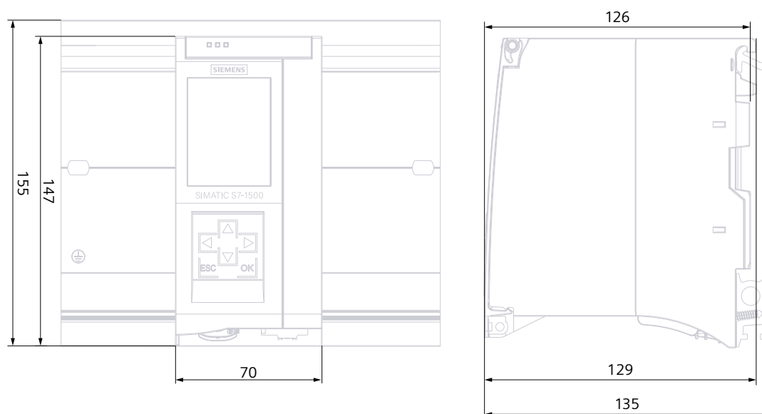
Figure A-1 Dimension drawing of CPU 1515-2 PN, front and side views
