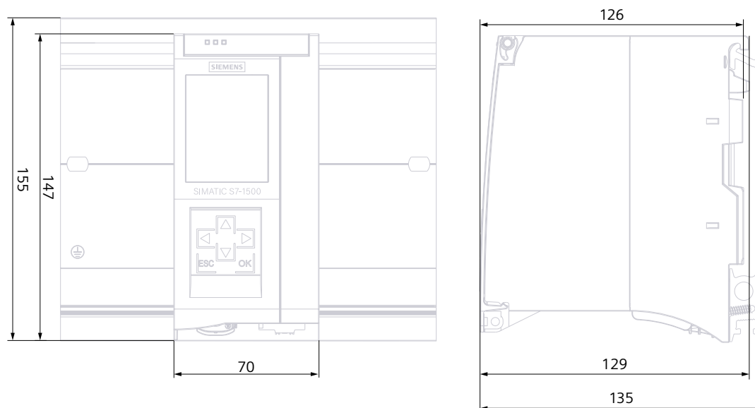
Figure A-1 Dimensional drawing of the CPU 1516-3 PN/DP
