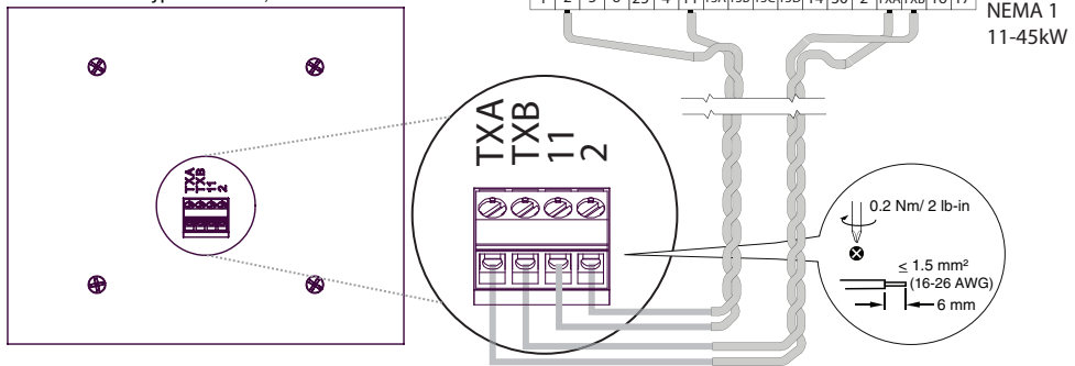
Remote Keypad installed, Rear View
