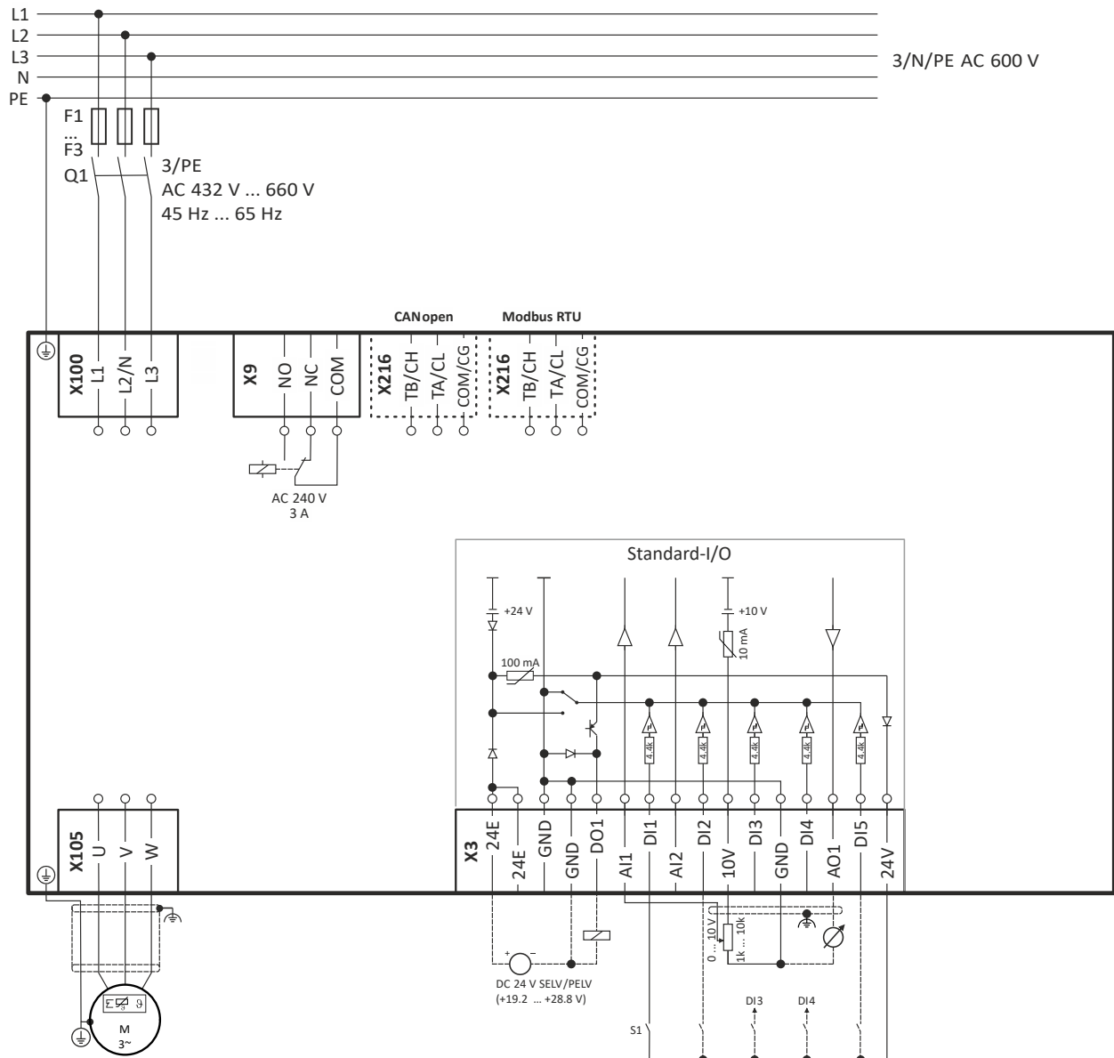
Fig. 7: Wiring example
