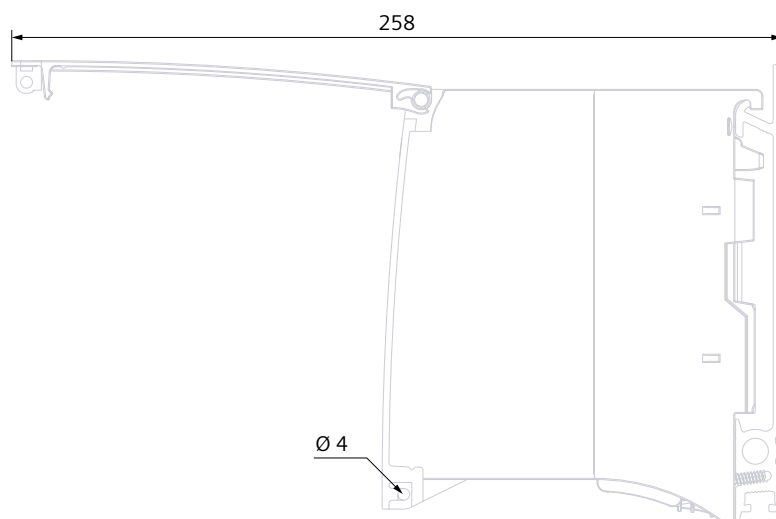
Figure A-2 Dimensional drawing CPU 1517-3 PN, side view with open front panel
