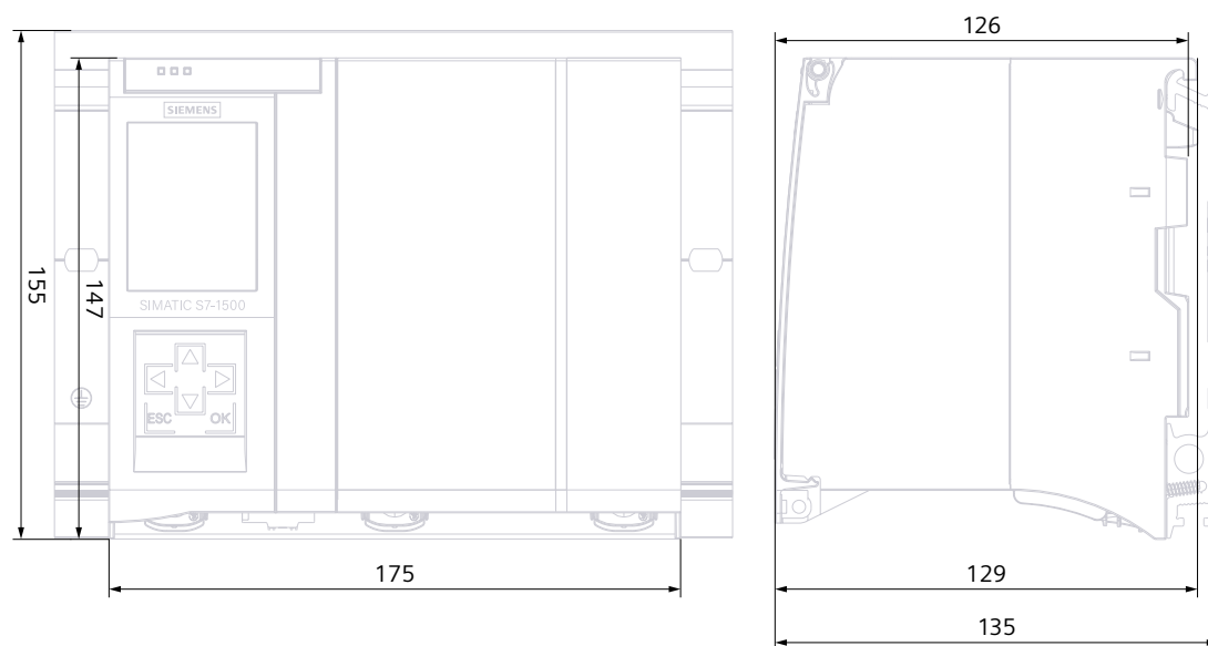
Figure A-1 Dimensional drawing of the CPU 1517-3 PN, front and side view
