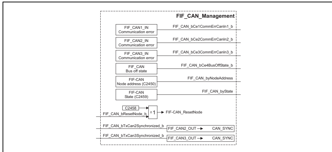
FIF_CAN_Managementsystem block
