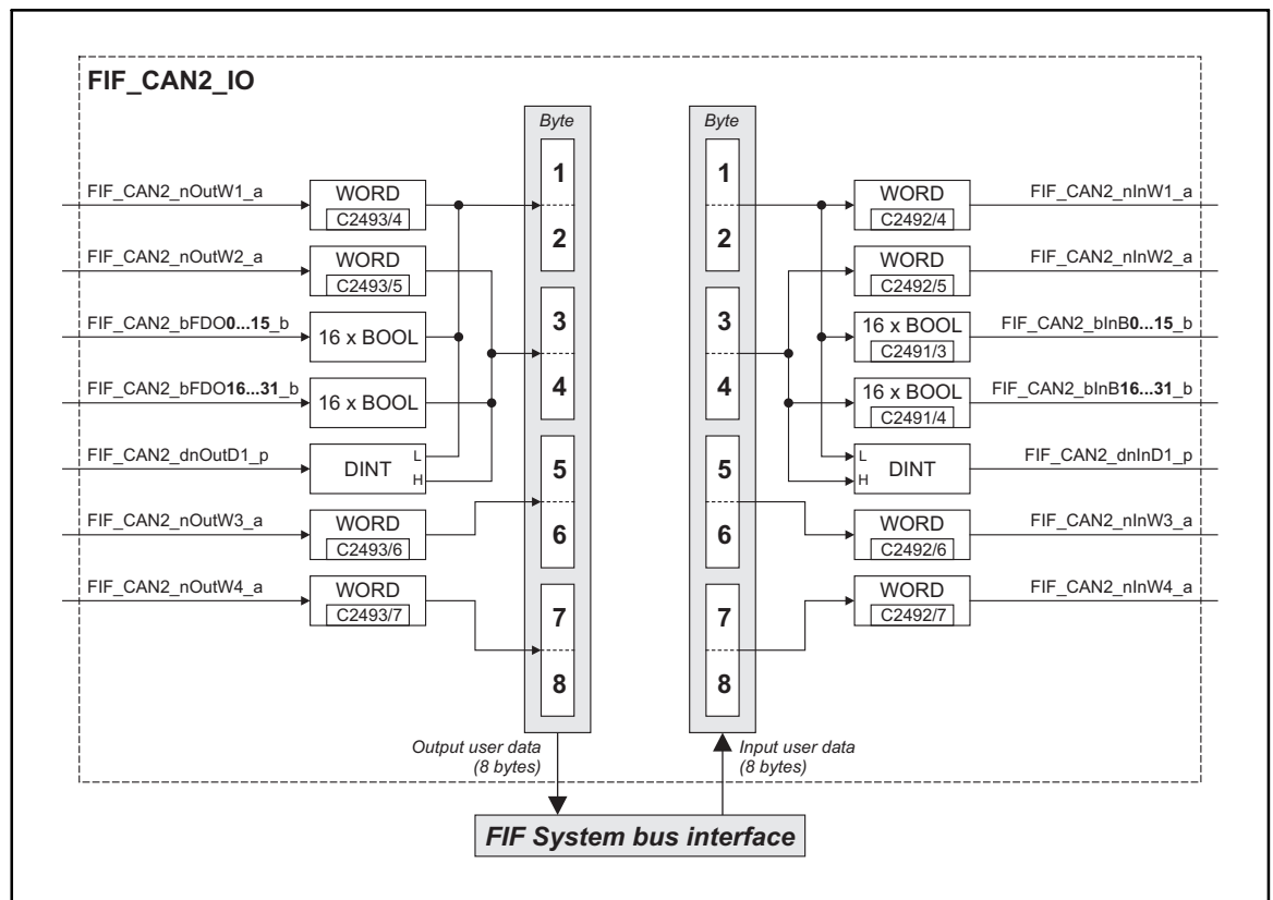
FIF_CAN2_IO system block
