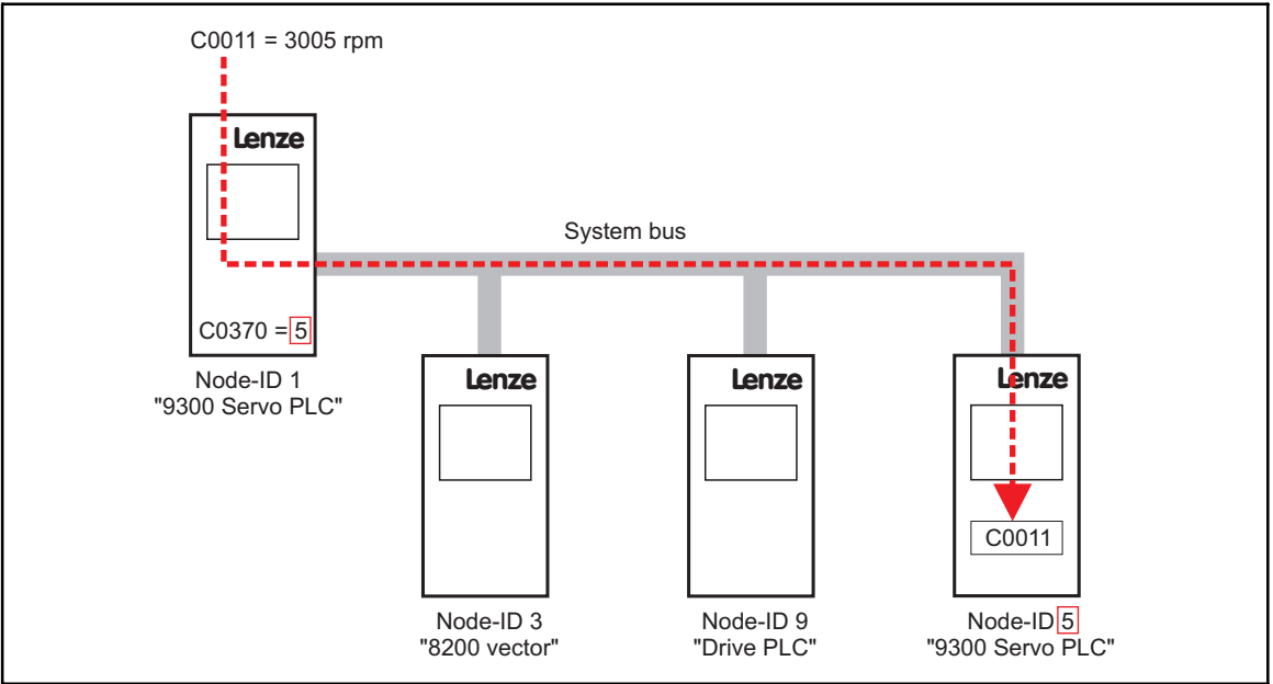
Fig. 3-3 Remote parameterisation (gateway function)
