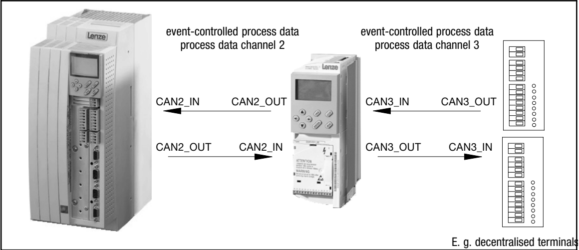
Fig. 2-3 Process data channels 2 and 3 (CAN2_IO/CAN3_IO) for the event- or time-controlled data exchange
