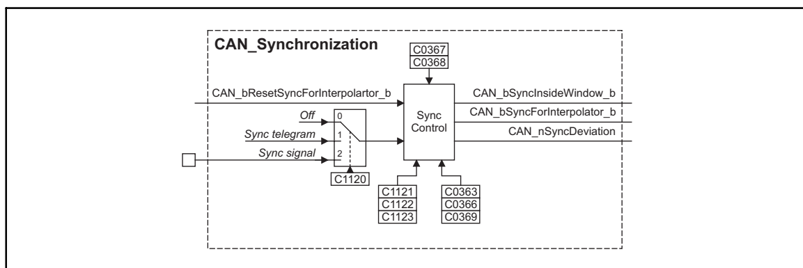
CAN_Synchronizationsystem block
