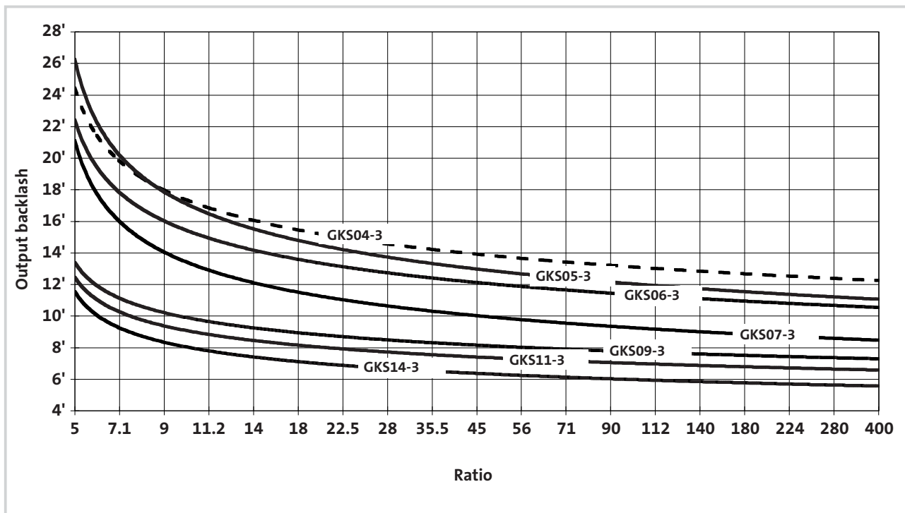
Helical-bevel gearbox GKS□□-3
