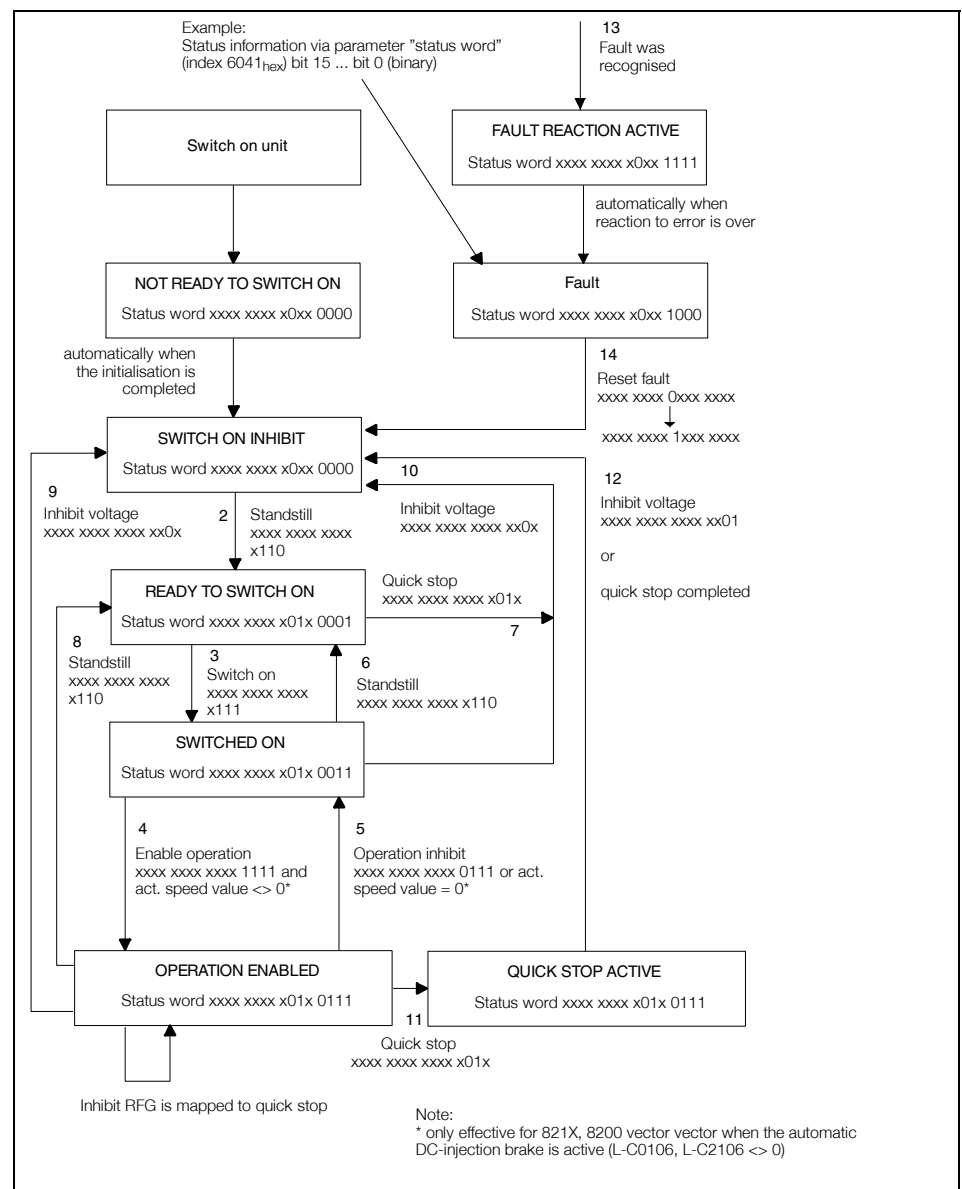
Fig. 5.6-10 Status diagram: DRIVECOM control
