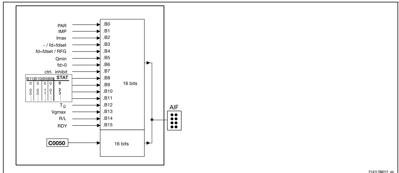
Fig. 5.6-1 Read access to status word and actual frequency in 82XX (fixed assignment)
