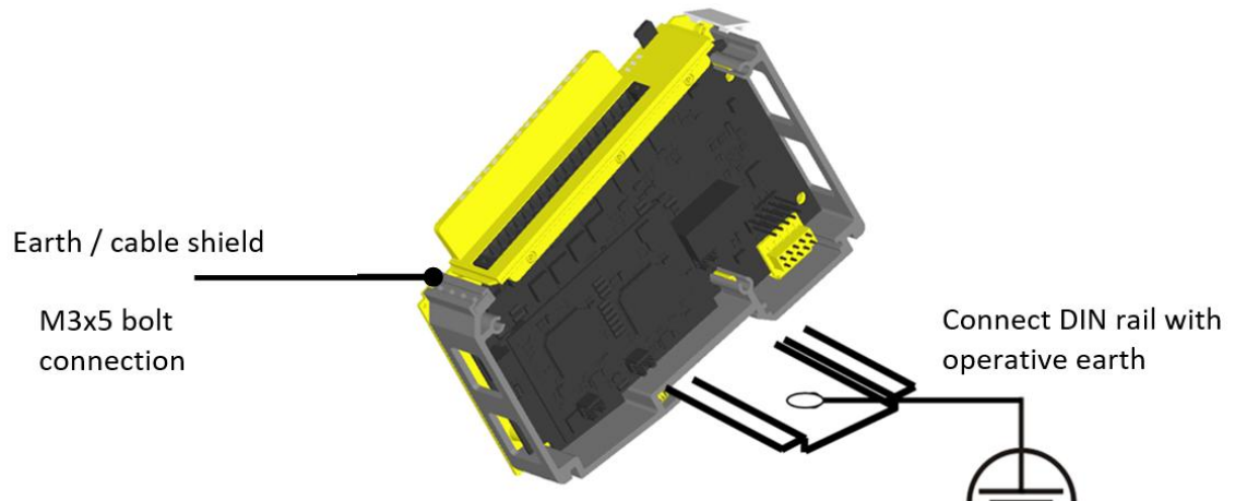
Figure 5: Aluminium profile in the Safety I/O-module
