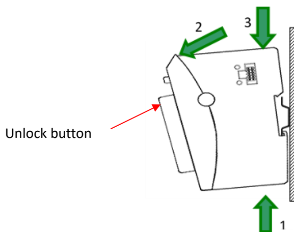
Figure 4: Uninstalling a module
