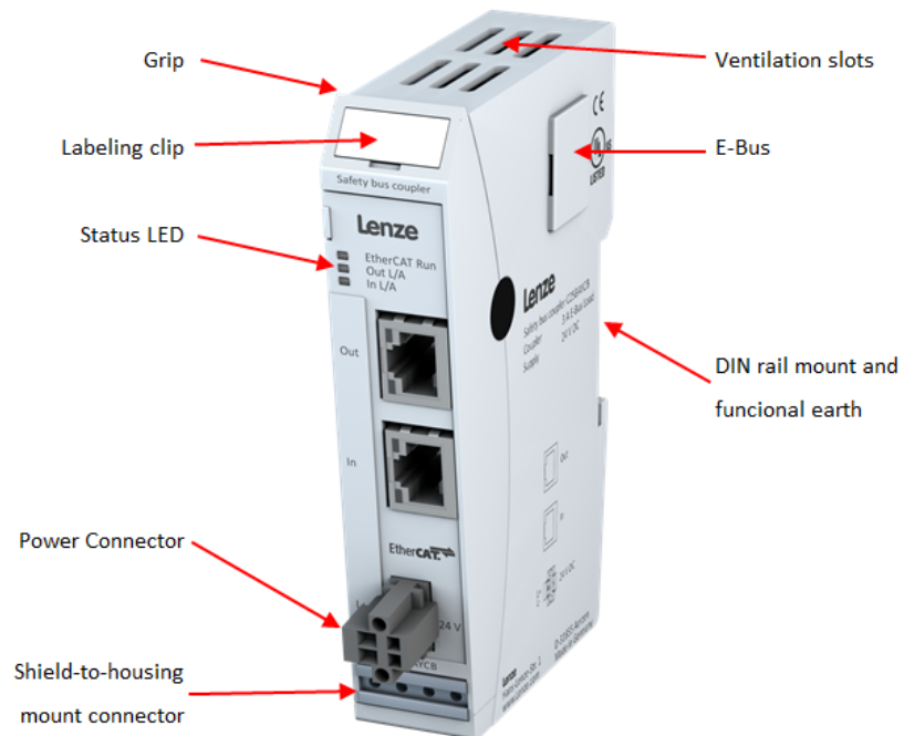
Figure 2 Module layout
