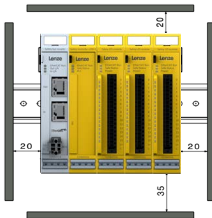
Figure 3: Installation position
