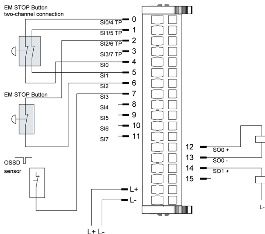
Figure 2: Example of how to wire the inputs and outputs
