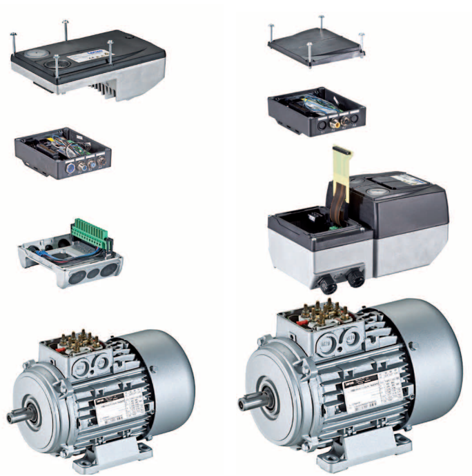
8400 motec 0.37至3.0 kW
