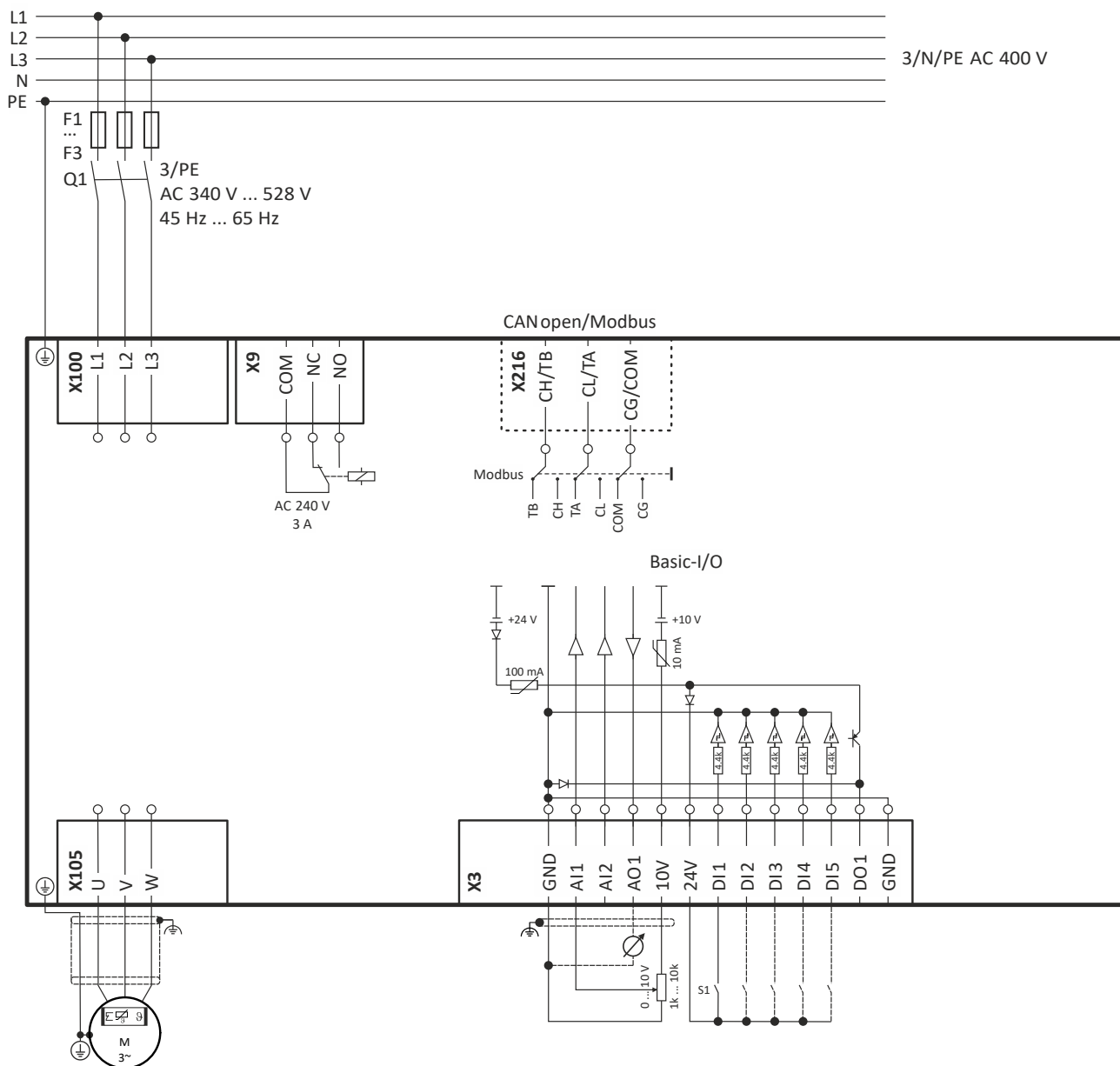
Fig. 5: Wiring example
