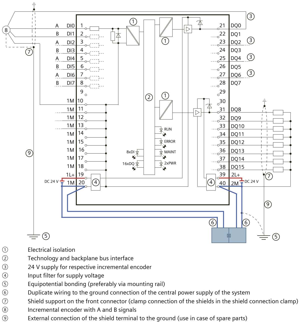
Figure 4-3 Block diagram with incremental encoders
