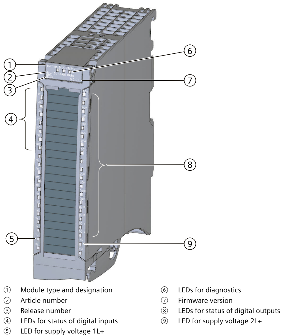
Figure 3-1 View of the TM Timer DIDQ 24x24V module
